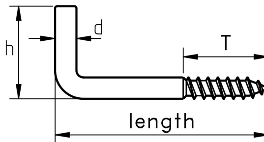
Figure 1: Square Hook with Wood Thread
