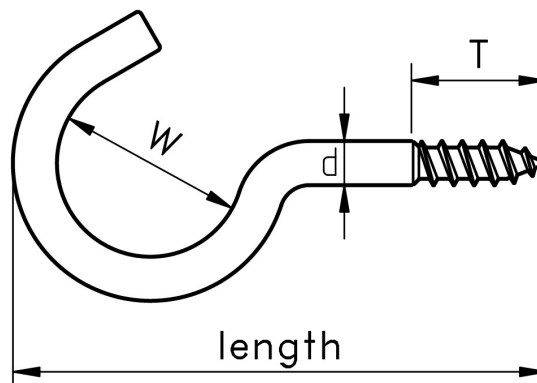
Figure 1: Cup Hook with Wood Thread
