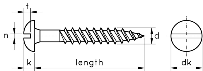
Figure 1: Slotted Round Head Wood Screw to British Standard BS 1210
