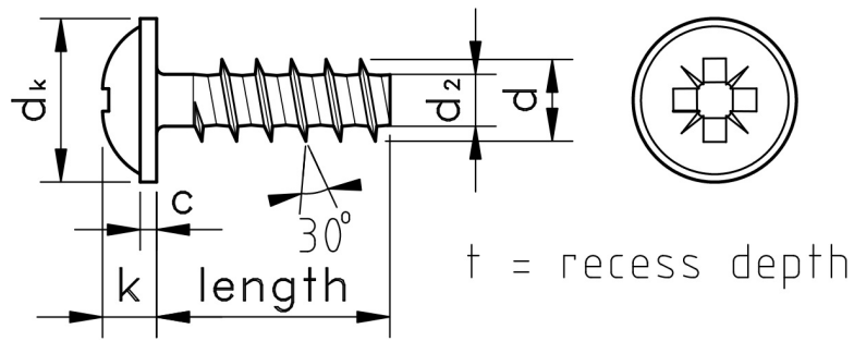
Figure 1: Pozi Pan Flange Thread Forming Screw for Plastics
