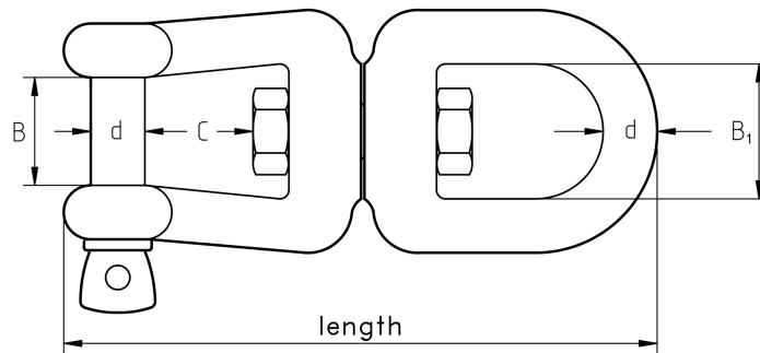
Figure 1: Swivel Shackle with Eye and Fork
