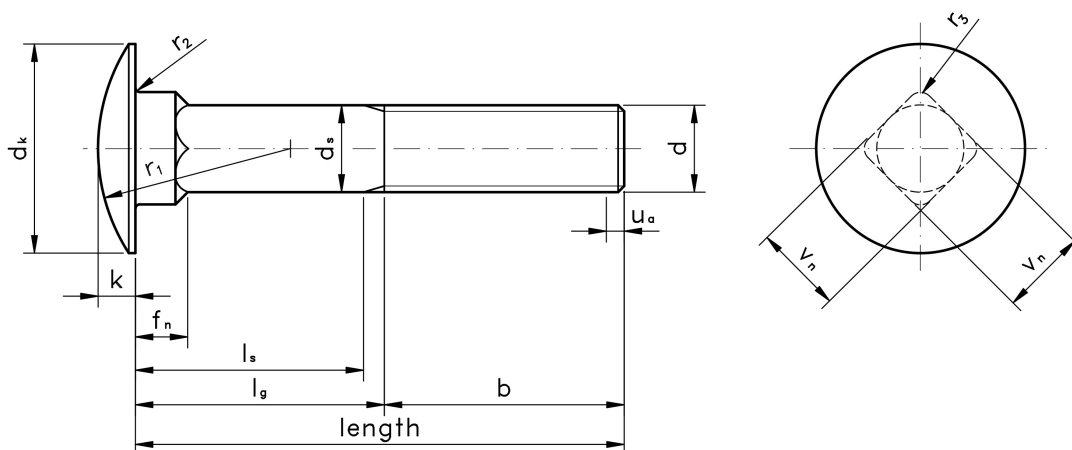
Figure 1: Coach Bolts with part thread
