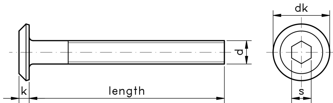
Figure 1: Metric Connector Bolts
