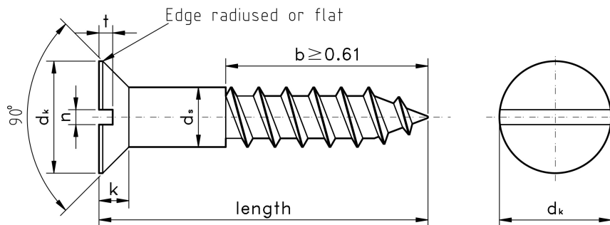
Figure 1: DIN 97 Slotted Countersunk Wood Screw
