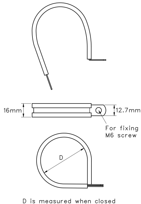
Figure 1: A4 Stainless Steel Rubber Lined P Clip
