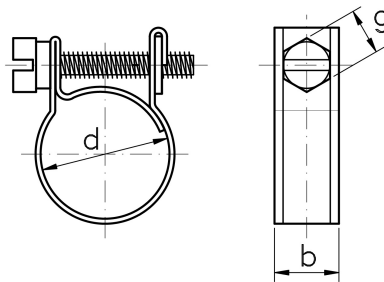
Figure 1: Mini Hose Clip in A2 Stainless Steel
