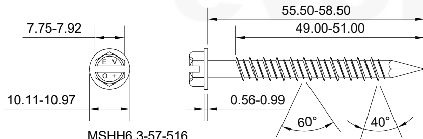
MSHH6.3-57-516
