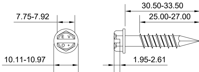
MSHH6.3-32-516
