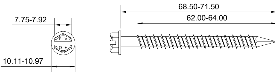
MSHH6.3-70-516
