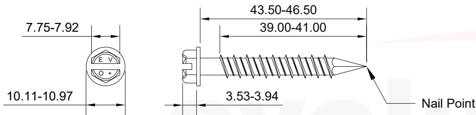
MSHH6.3-45-516
